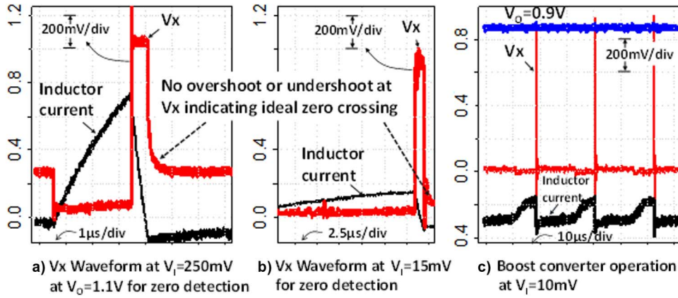
Fig. 18. Inductor switching waveforms: (a) V_x at V_I = 250 \text{ mV} and (b) V_I = 15 \text{ mV} showing near ideal zero crossing. (c) Switching operation at 10 mV.
