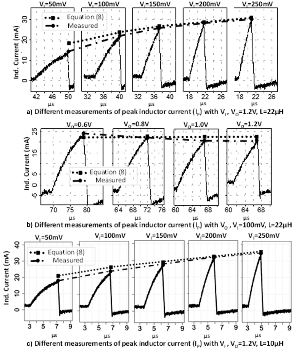
Fig. 10. Measurement results of peak inductor current: (a) variation with V_I with L = 22 \mu H , (b) variation with V_O with L = 22 \mu H , and (c) variation with V_I with L = 10 \mu H shows that the LS control circuit tracks I_P based on (8) for maximum efficiency.
